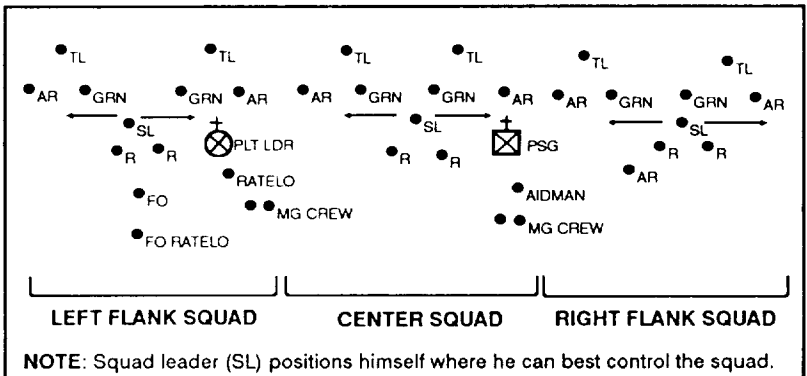
Figure 2-12. Platoon-line, squads-on-line.
